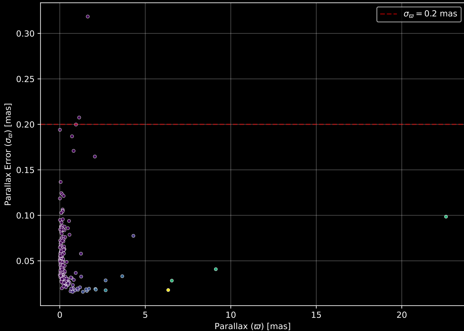
APOGEE DR17 Field: [006+02] Parallax Quality (n= 215)
