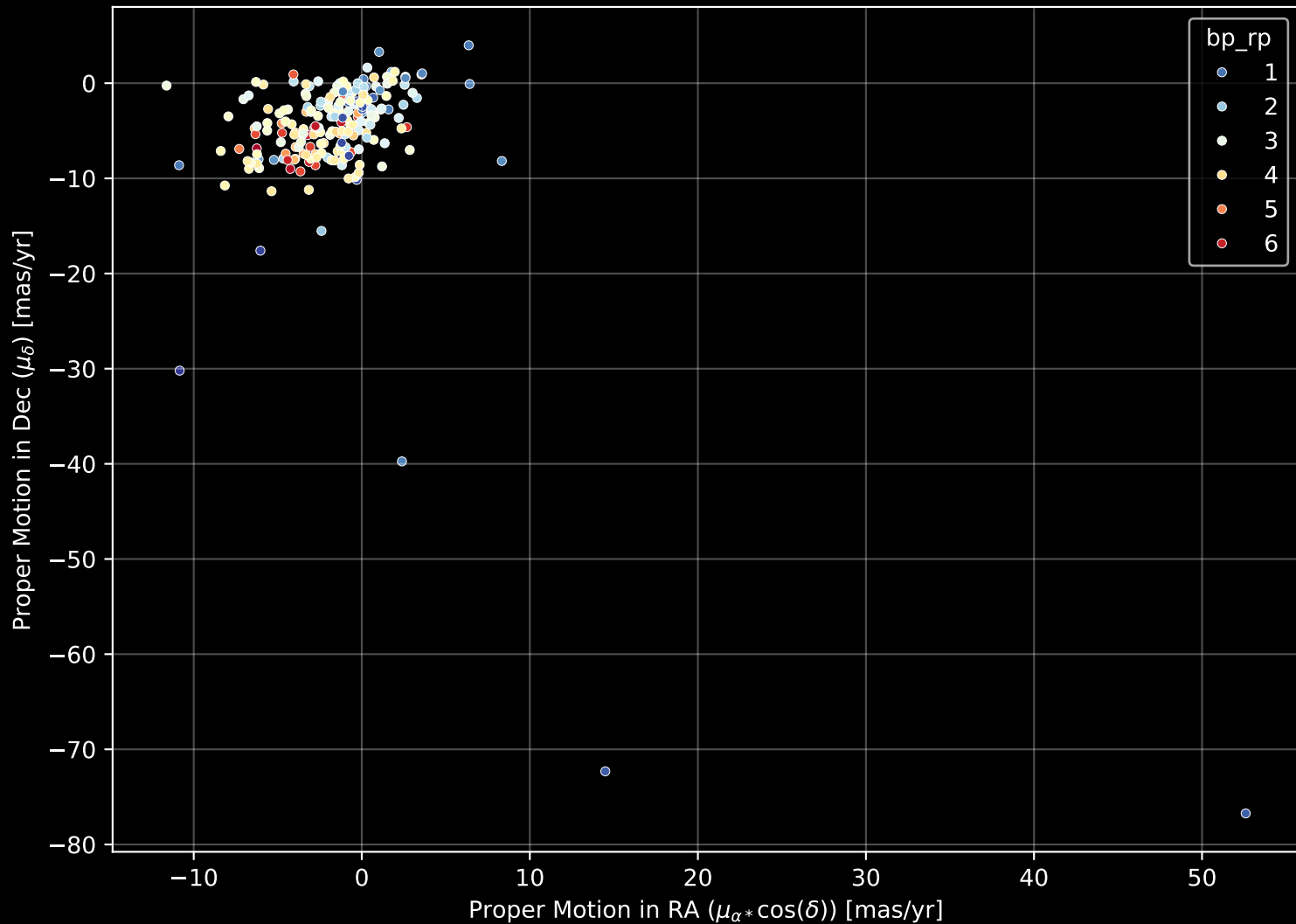
APOGEE DR17 Field: [006+02] Proper Motion Diagram (n= 215)
