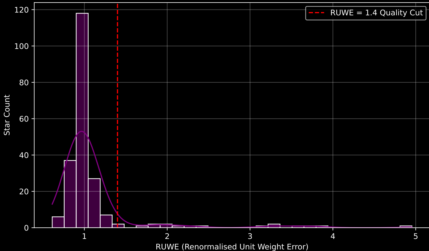
GAPOGEE DR17 Field [006+02] RUWE Distribution (n= 212)
