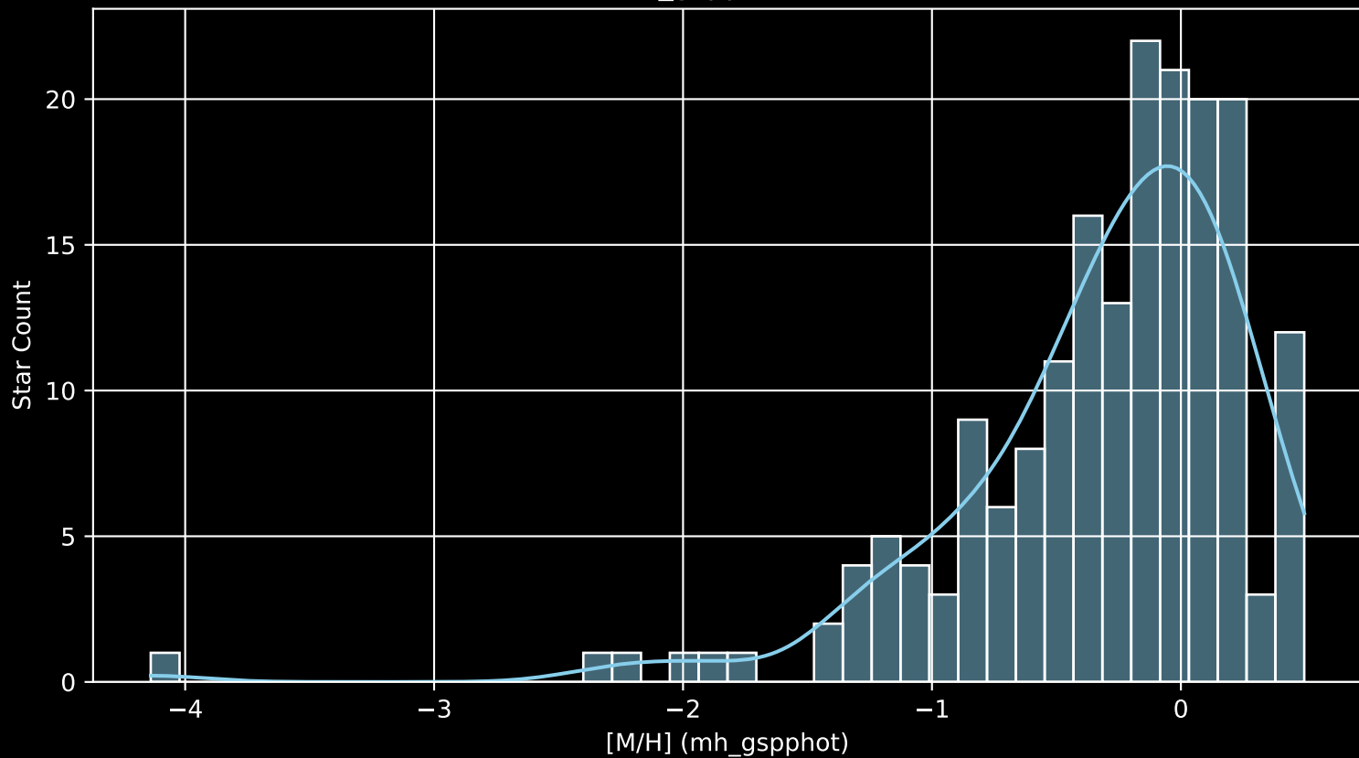
APOGEE DR17 Field: [006+02 [M/H] (mh_gspphot) (n= 185)
